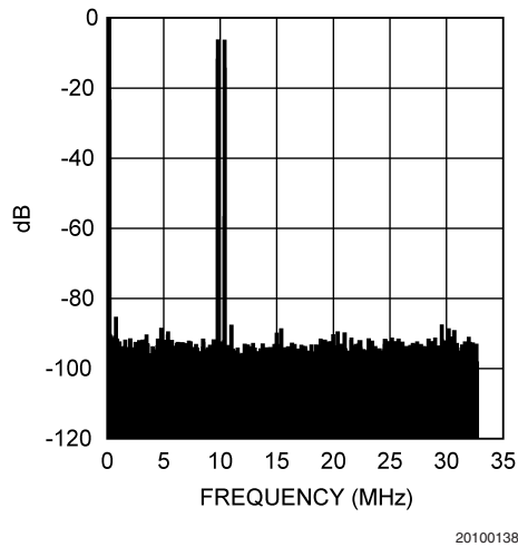
Intermodulation Distortion, f_{IN1} = 9.6 MHz, f_{IN2} = 10.2 MHz
